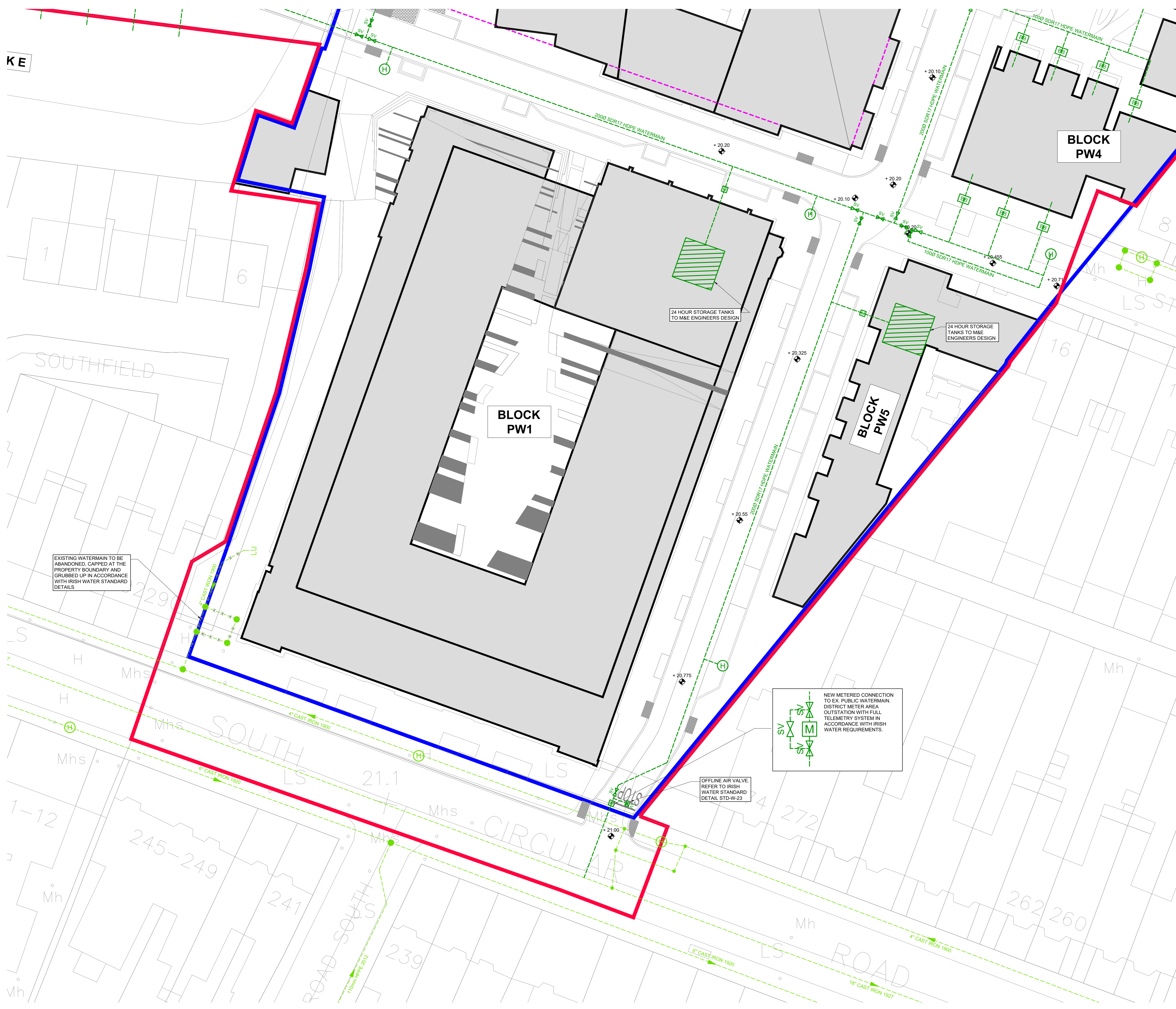
PROPOSED WATERMAIN LAYOUT - SHEET 2 SCALE @ A2: 1:500
